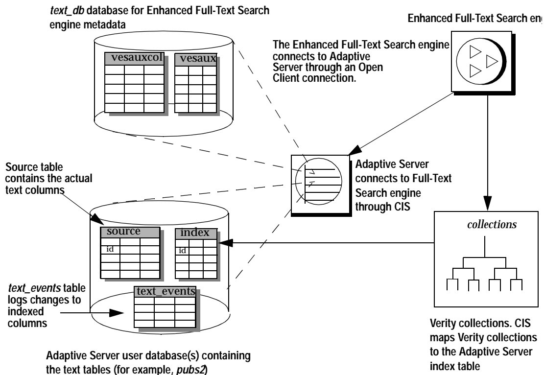
Figure 2-1: Components of the Enhanced Full-Text Search engine
